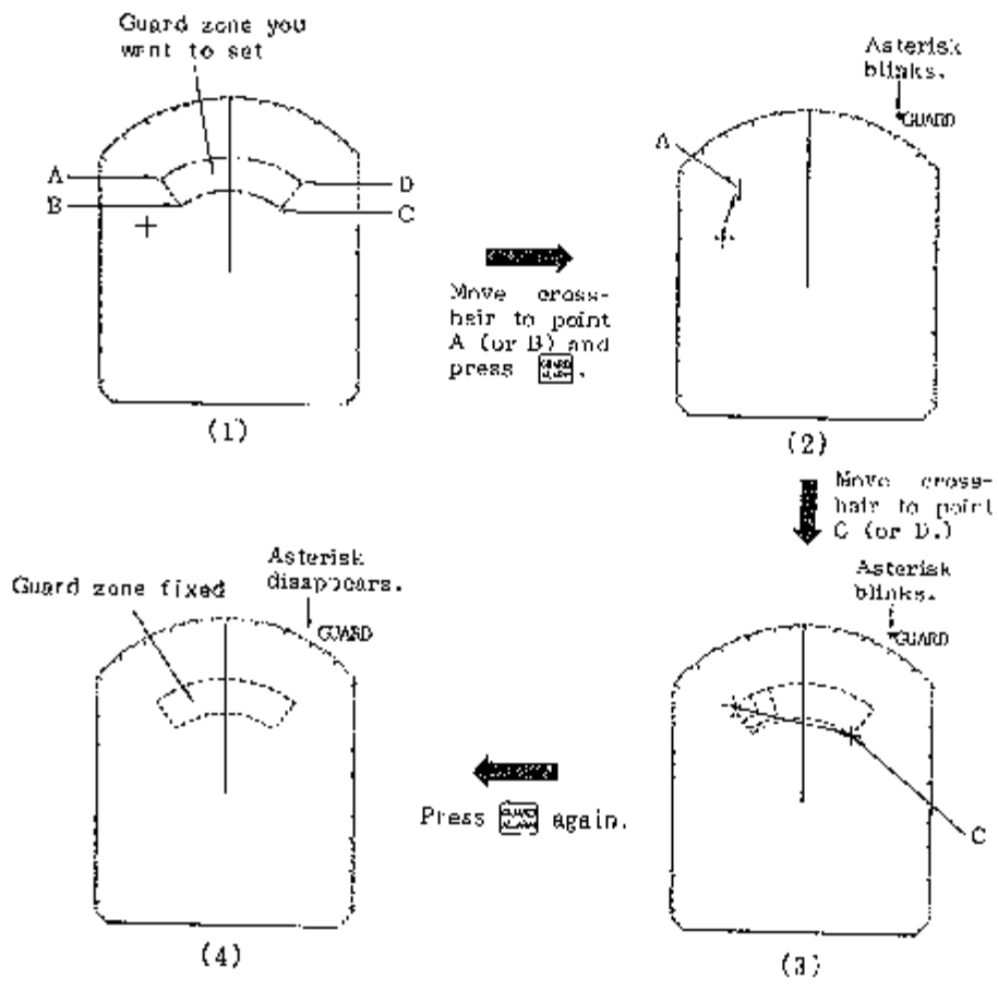
Fig.30 Setting Guard Zone
