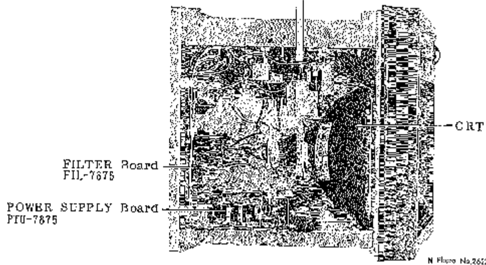
Fig.51 Display Unit Top View
