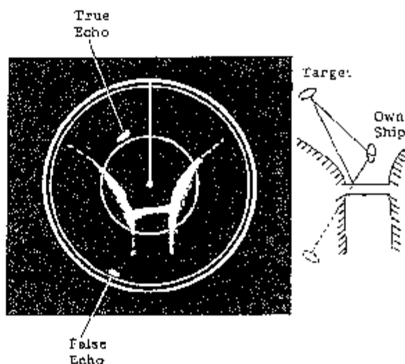
Fig.43 Indirect Echoes
