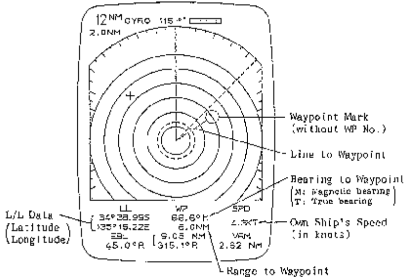
Fig.34 Nav Data on the Screen
