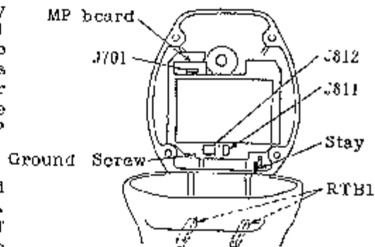
Fig.9 Internal Wirings
