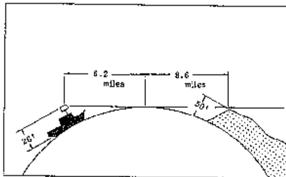
Fig.38 Radar Horizon
