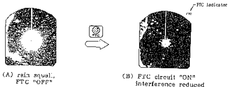
Fig.28 Precipitation Interference
