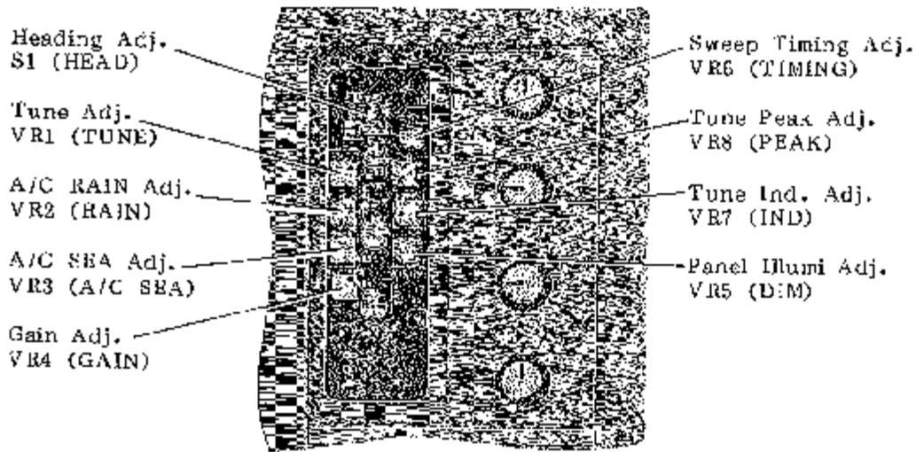
Potentiometer Compartment
